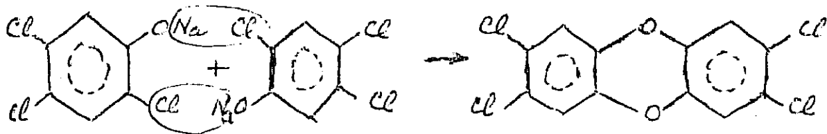
TCDD (dioxine)
